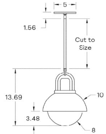
Dimensional Drawing
