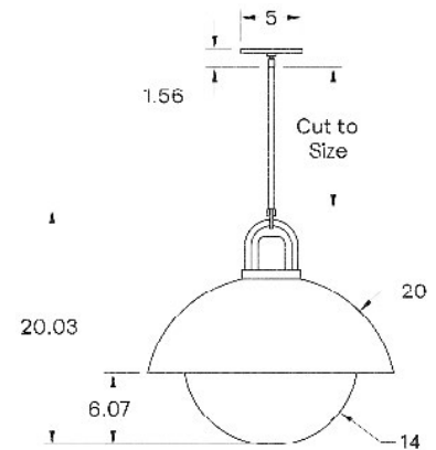
Dimensional Drawing
