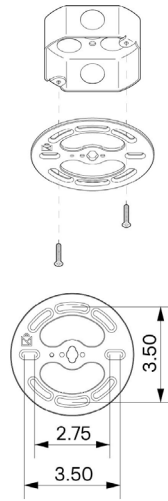
Mounting Drawing
