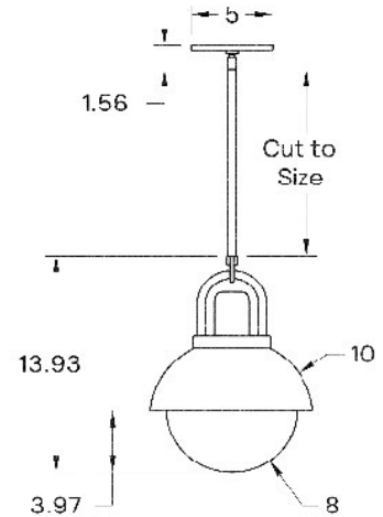
Dimensional Drawing
