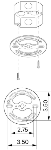
Mounting Drawing
