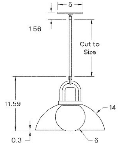
Dimensional Drawing
