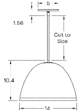
Dimensional Drawing
