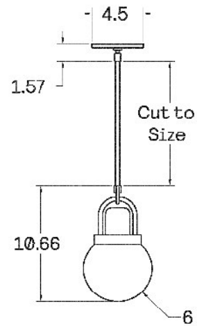
Dimensional Drawing
