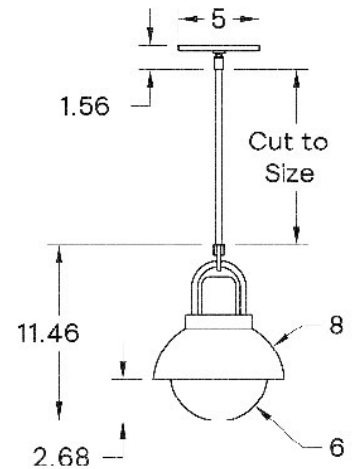
Dimensional Drawing
