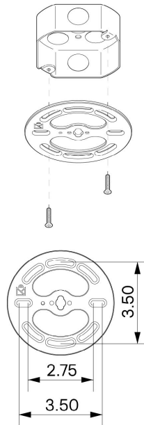
Mounting Drawing
