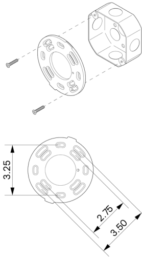
Mounting Drawing
