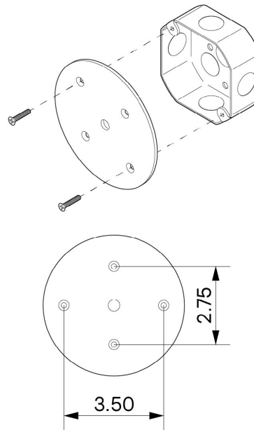
Mounting Drawing
