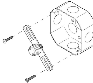
Mounting Drawing
